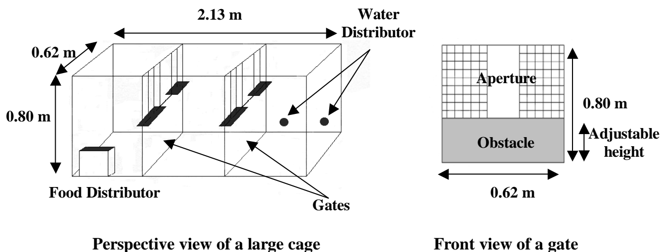
Figure 1. Illustration of a large cage equipped with two gates comprising an obstacle adjustable in height.
